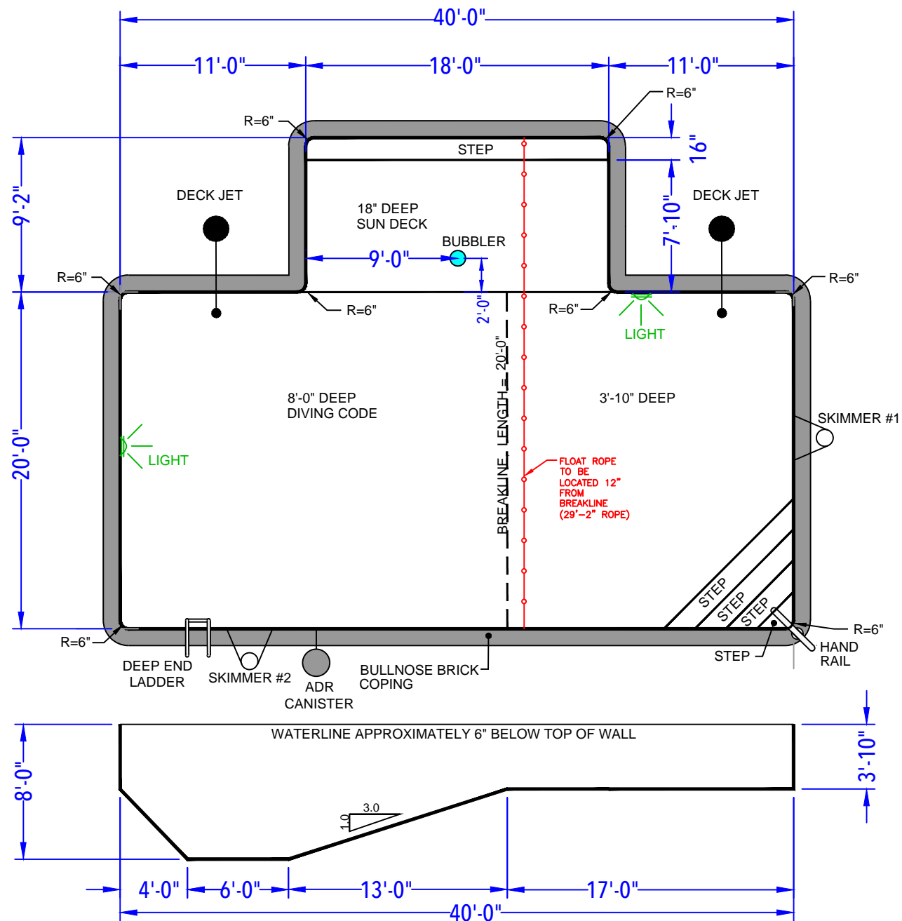
DEPTH DETAIL
