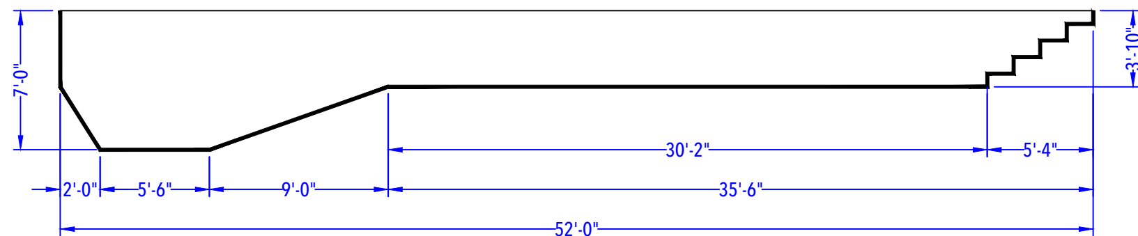
DEPTH DETAIL
