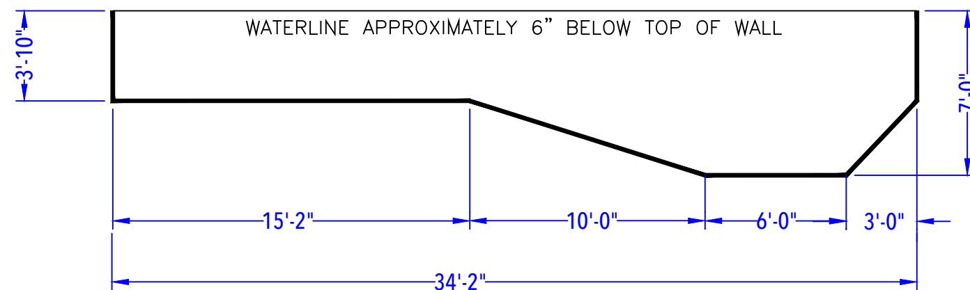
DEPTH DETAIL
