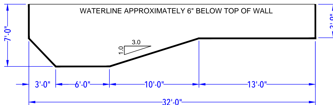
DEPTH DETAIL
