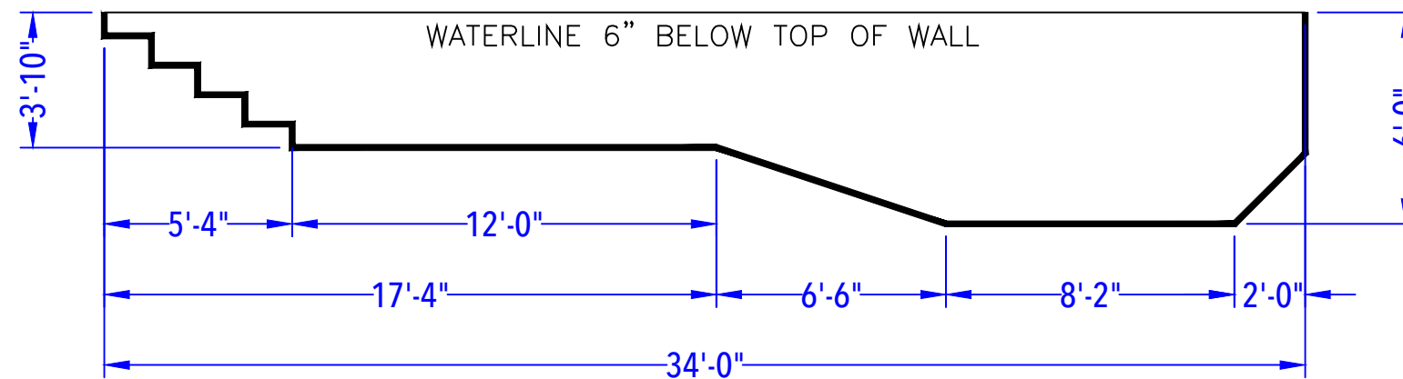
DEPTH DETAIL
