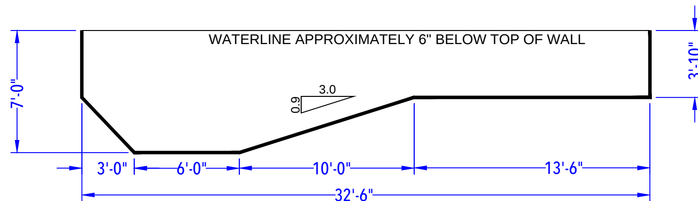
DEPTH DETAIL
