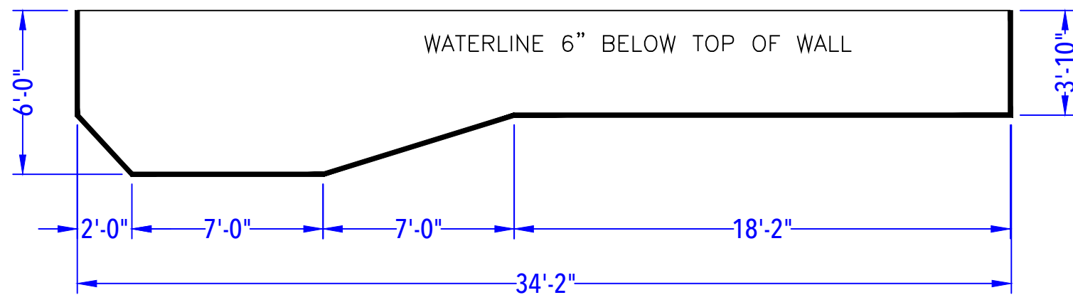
DEPTH DETAIL
