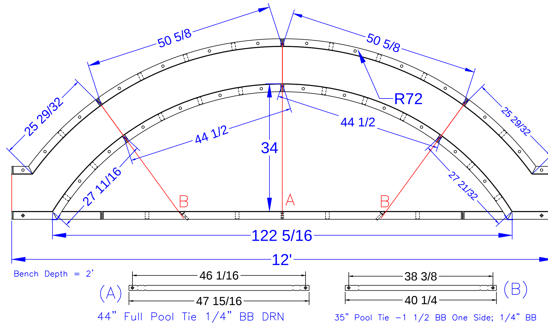
10'-2" ROMAN END LOVE SEAT (6' RADIUS)
