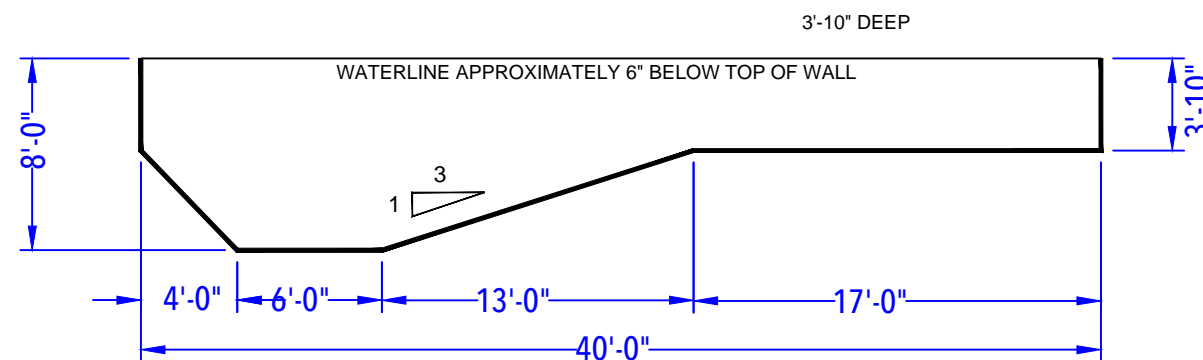
DEPTH DETAIL
