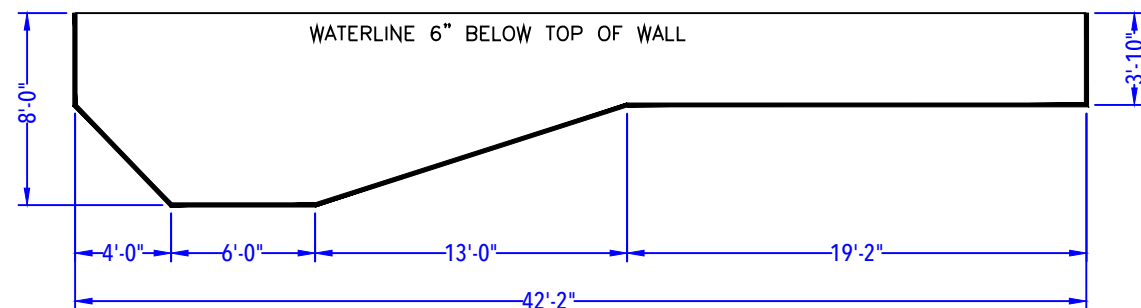
DEPTH DETAIL
