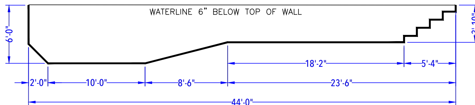
DEPTH DETAIL
