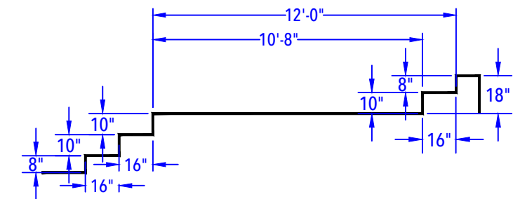
SUN DECK & ENTRY STEP DETAIL (After Concrete & Liner) N.T.S.
