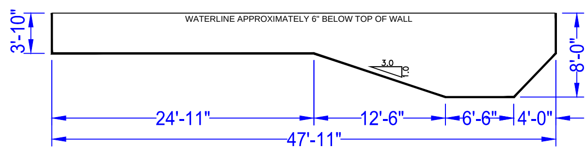
DEPTH DETAIL
