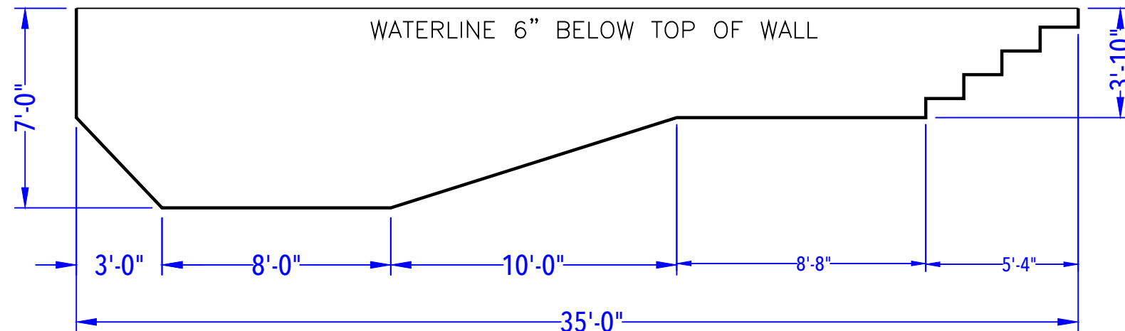
DEPTH DETAIL
