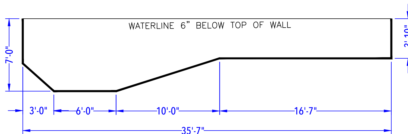
DEPTH DETAIL
