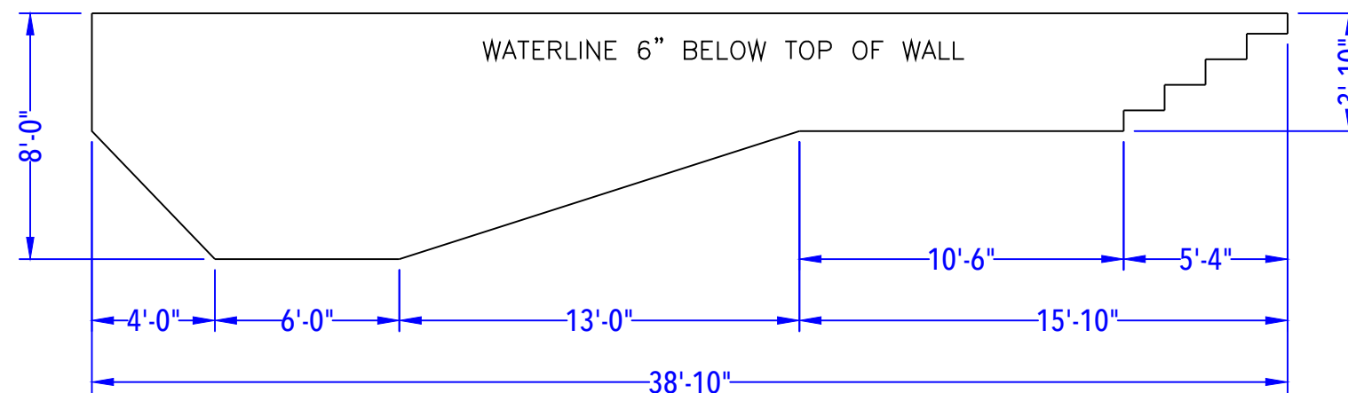
DEPTH DETAIL
