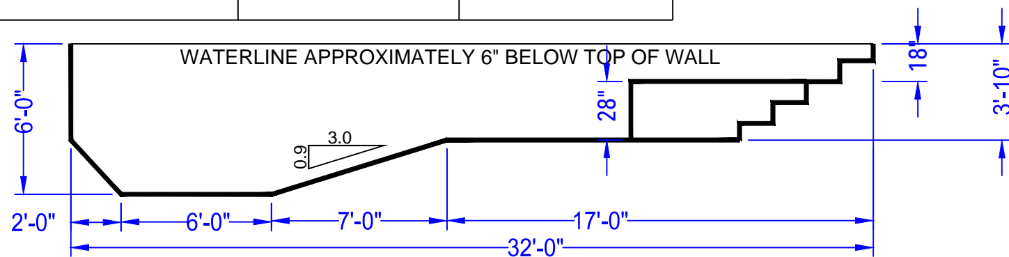
DEPTH DETAIL
