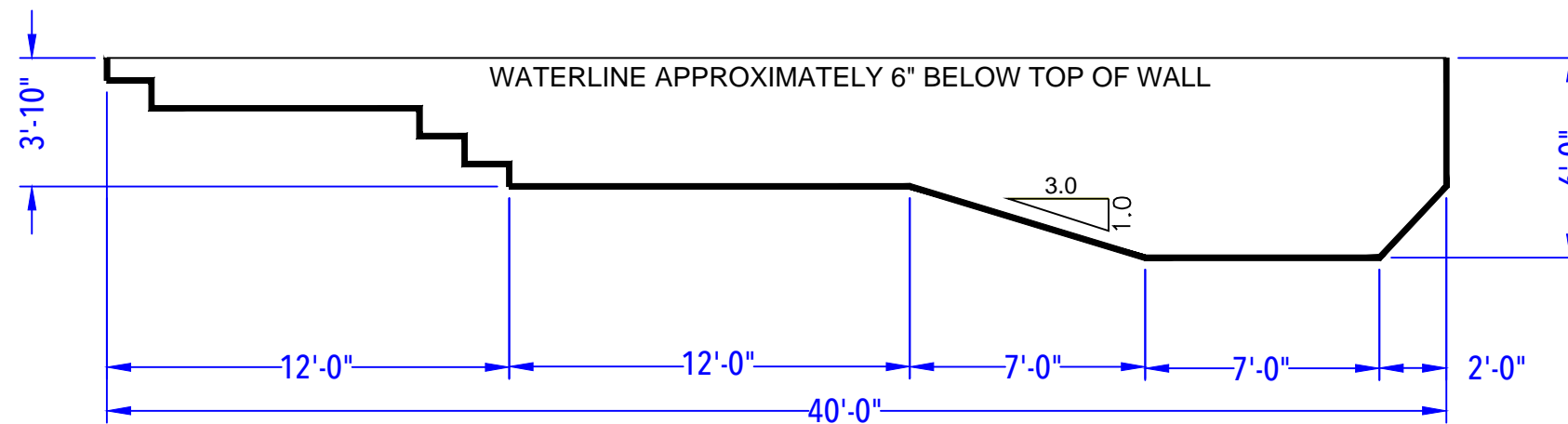
DEPTH DETAIL
