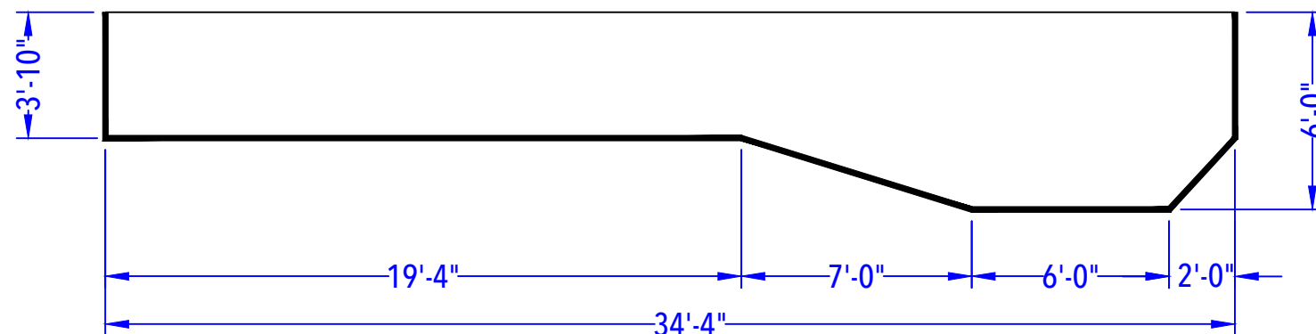
DEPTH DETAIL
