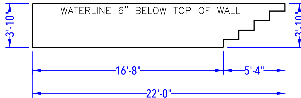
DEPTH DETAIL
