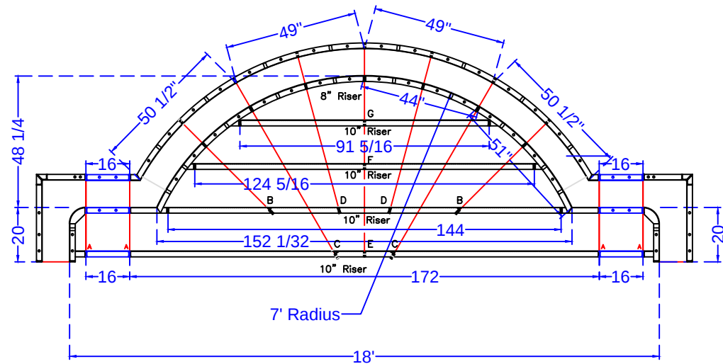
18' ROMAN END STEP ASSEMBLY SHOWN x 48 SCALE: 1' = 1/4"
