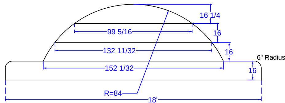
STEP DETAIL SCALE: 1' = 1/4"
