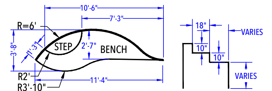
DEEP END BENCH & STEP OUT DETAIL (After Concrete & Liner) N.T.S.
