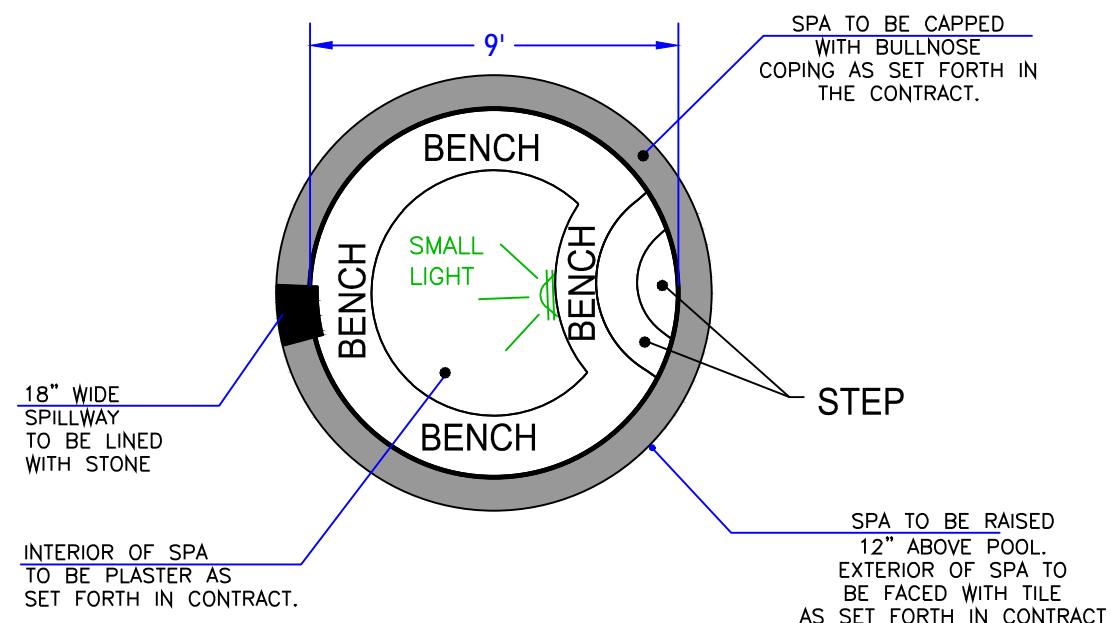
SPA PLAN VIEW (After Concrete & Plaster) N.T.S.
