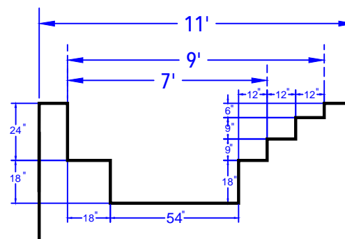
SPA ELEVATION VIEW (After Bottom & Liner) N.T.S.
