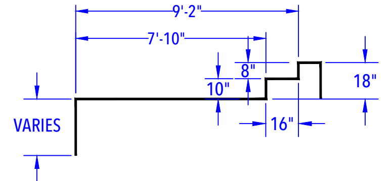
SIDE SUN DECK DETAIL (After Concrete & Liner) N.T.S.
