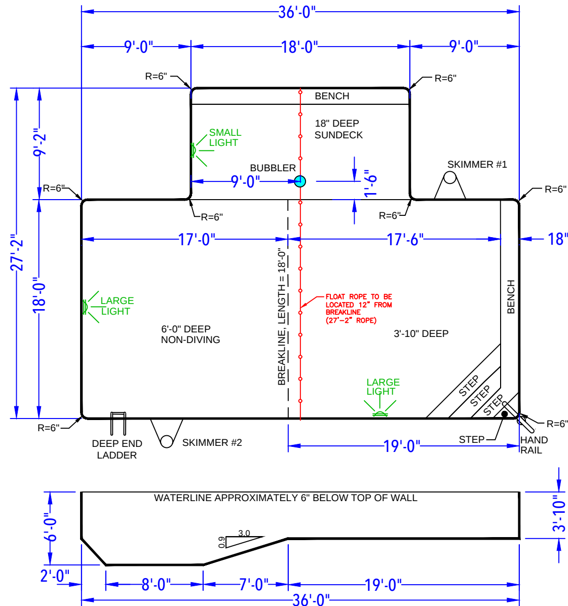
DEPTH DETAIL
