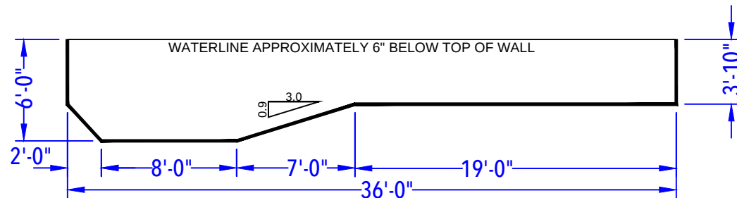
DEPTH DETAIL
