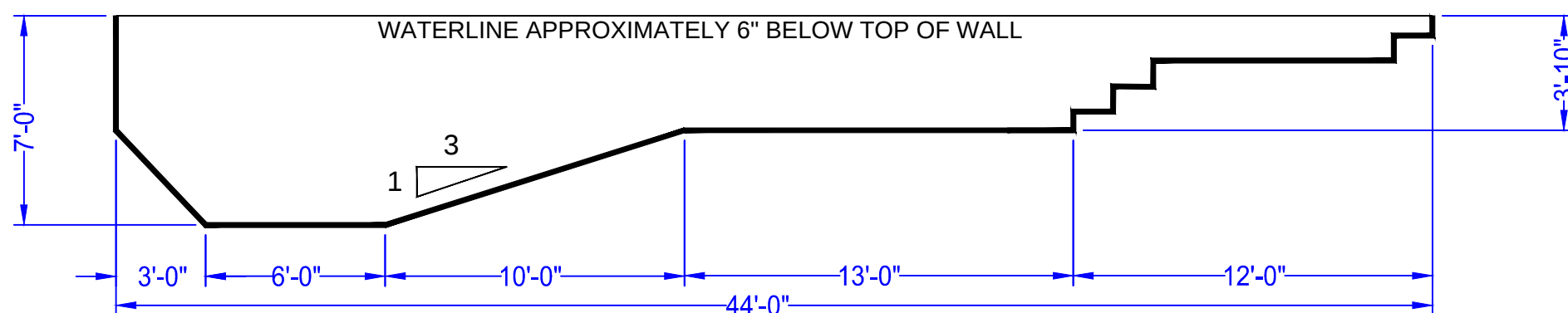
DEPTH DETAIL
