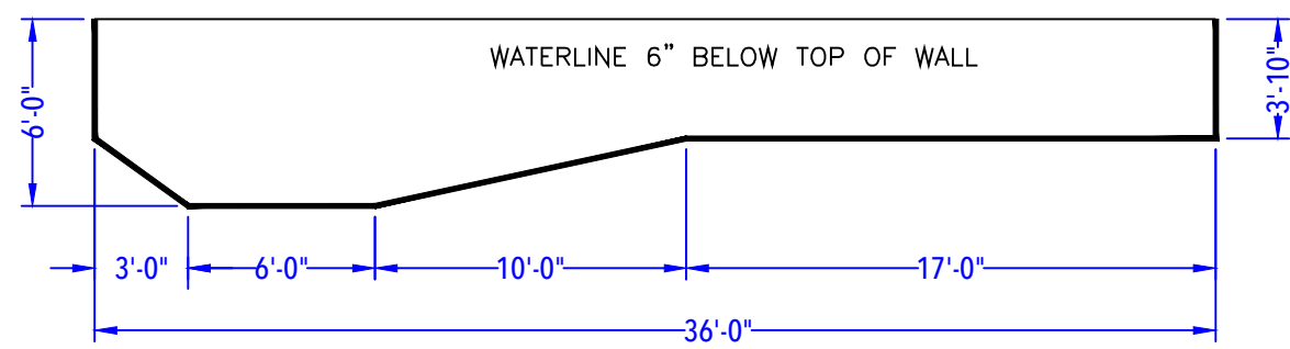
DEPTH DETAIL
