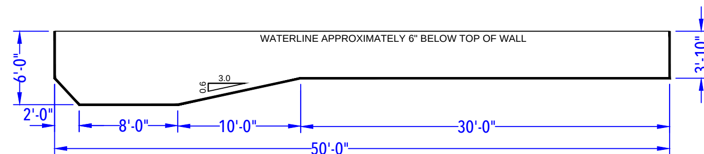
DEPTH DETAIL
