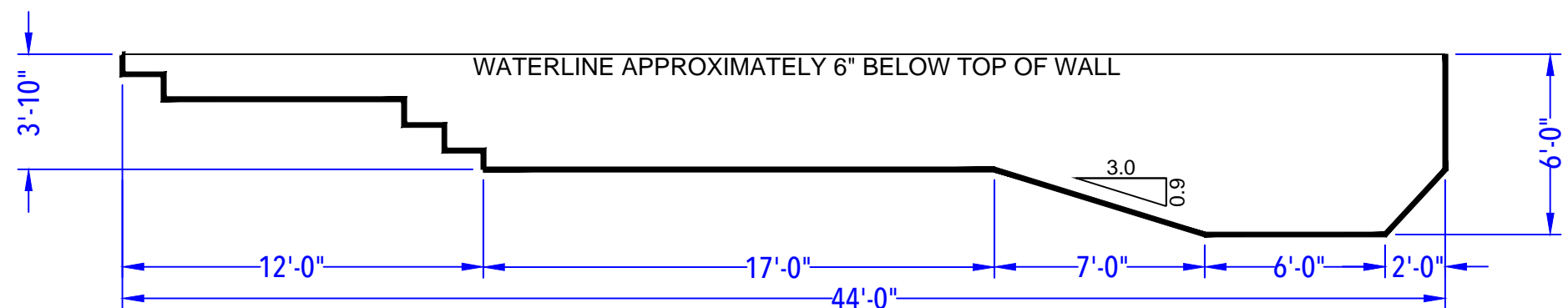
DEPTH DETAIL
