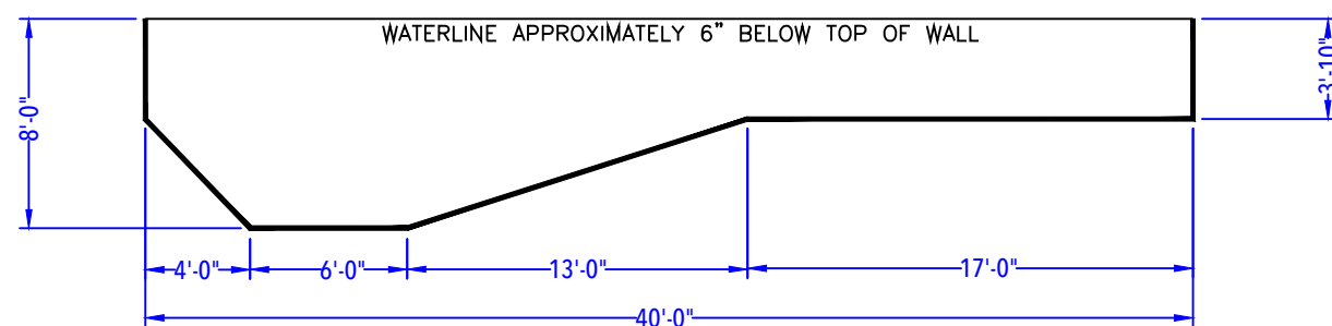
DEPTH DETAIL
