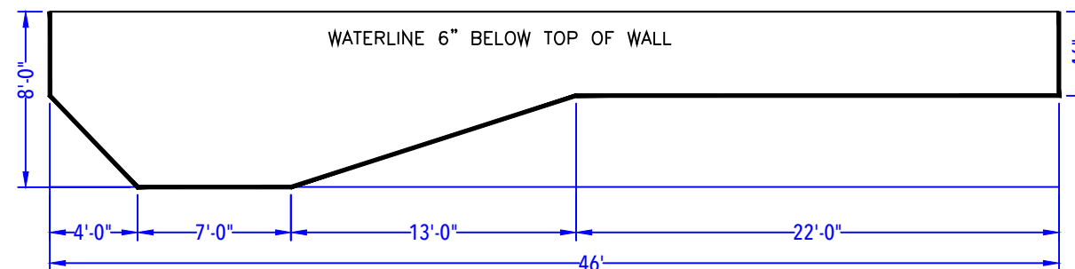
DEPTH DETAIL
