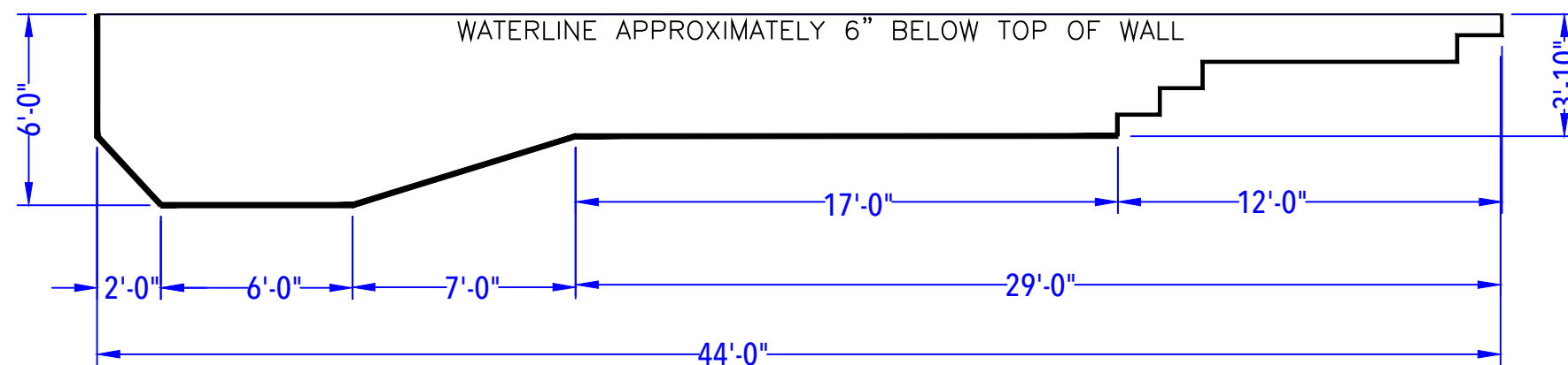
DEPTH DETAIL
