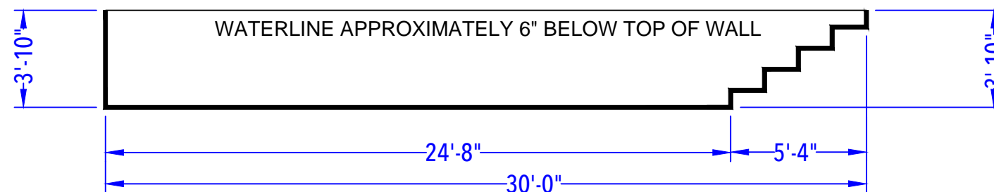
DEPTH DETAIL
