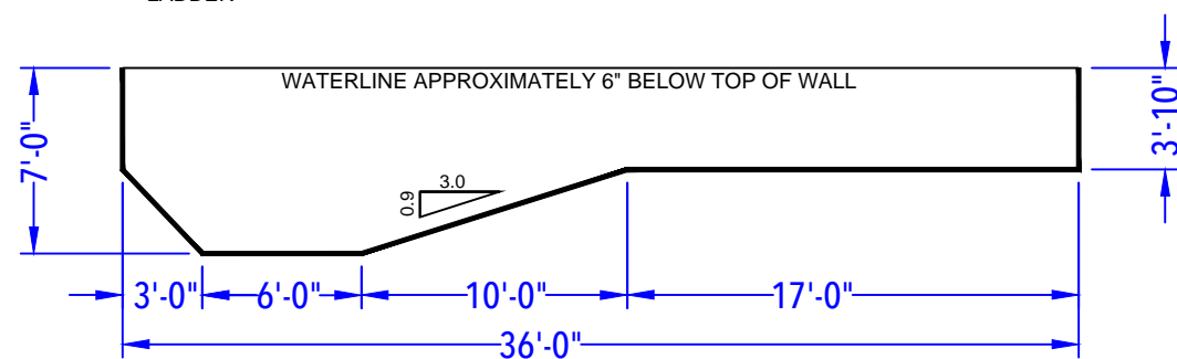
DEPTH DETAIL
