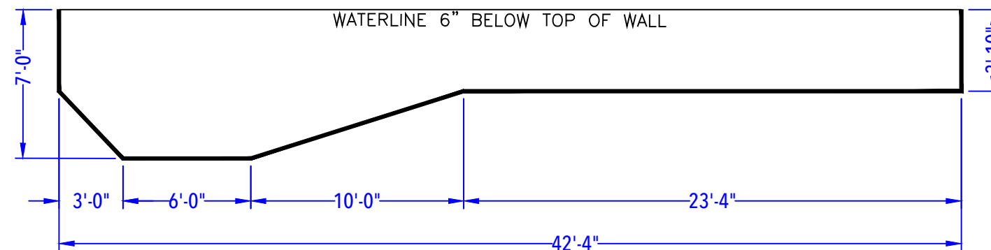
DEPTH DETAIL
