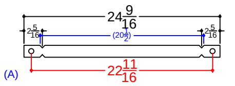
Qty(2) 20 1/2" Wall Tie - 2 Top Riser Overall Length Set 24 9/16" 8.28 ③
