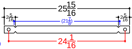
Qty(12) 21 7/8" Wall - 22" Full Tie - 2 Top Riser Overall Length Set 25 15/16" 8.74 ③
