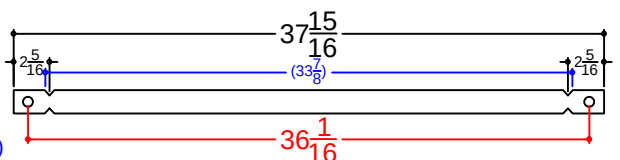
Qty(12) 33 7/8" Wall - 34" Full Tie - 2 Top Riser Overall Length Set 37 15/16" 9.55 ④
