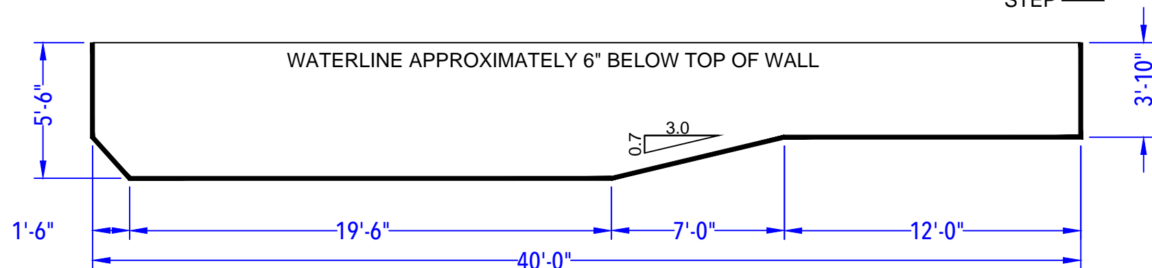
DEPTH DETAIL
