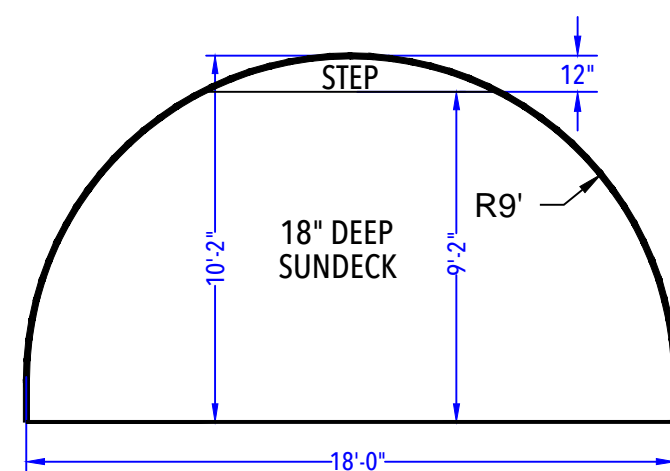
ENTRY STEP DETAIL (After Concrete & Liner) N.T.S.
