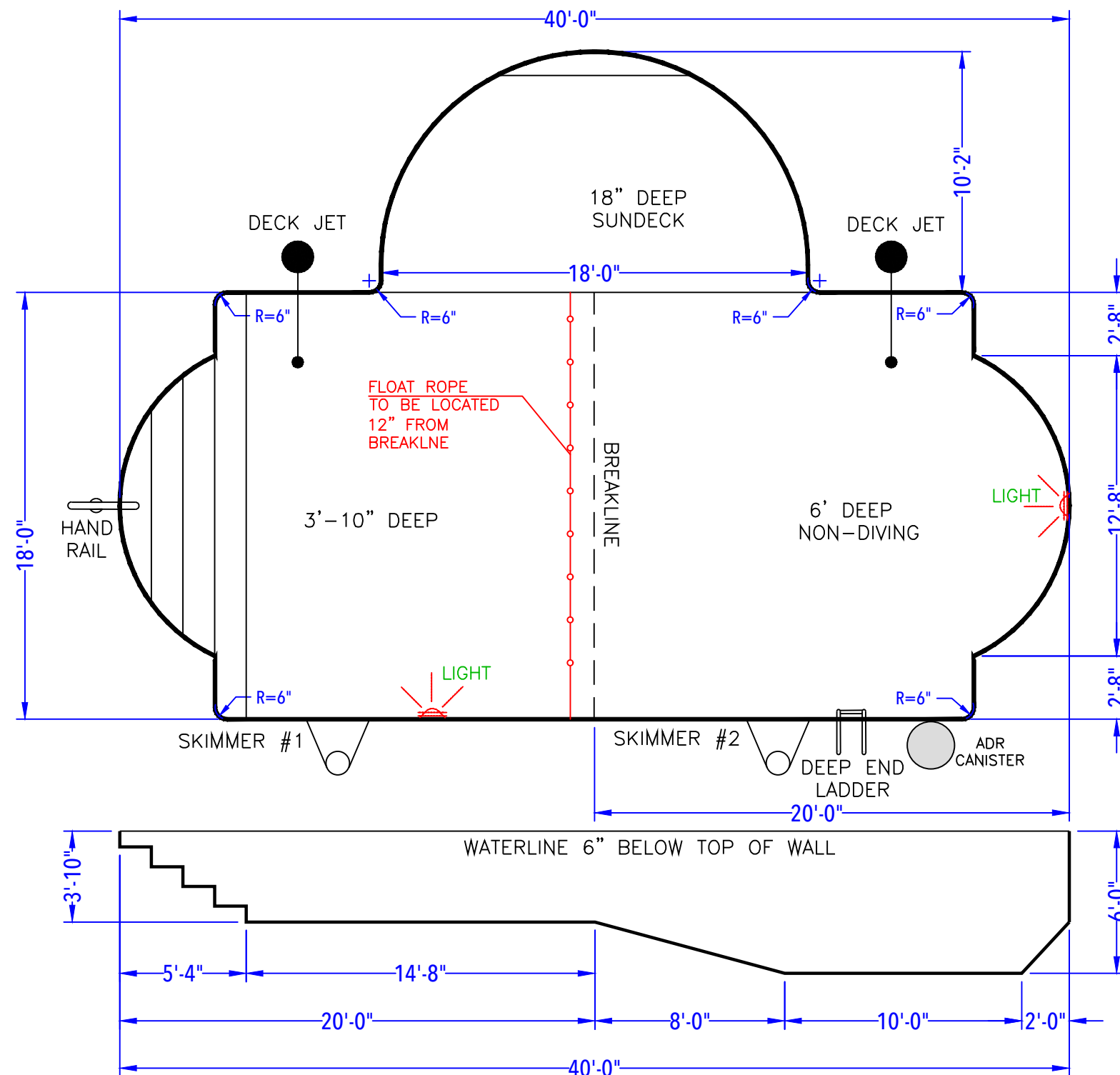
DEPTH DETAIL
