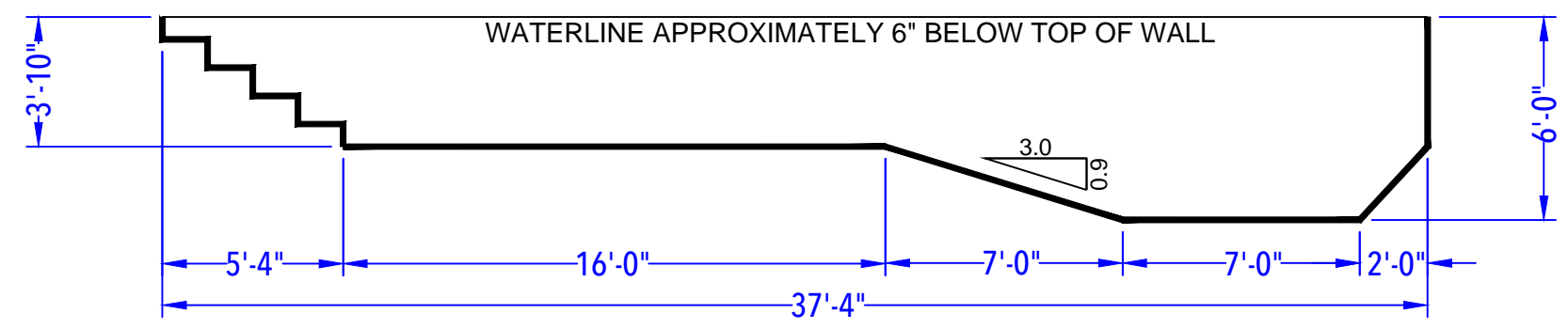
DEPTH DETAIL
