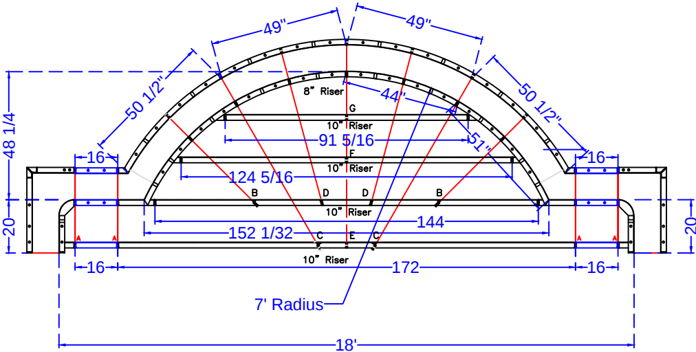
18' ROMAN END STEP ASSEMBLY SHOWN x 48 SCALE: 1' = 1/4"
