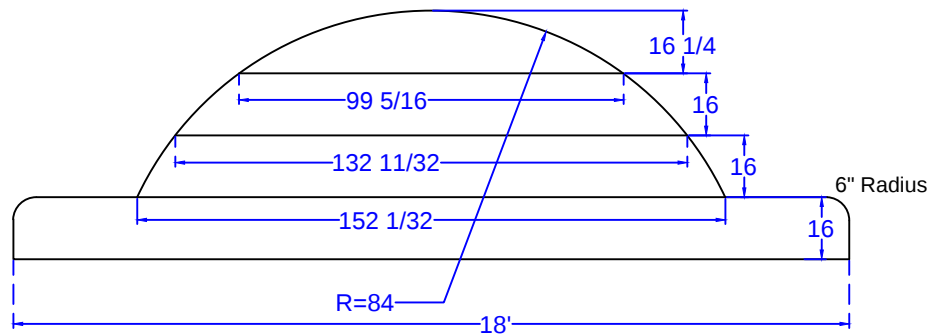
STEP DETAIL SCALE: 1' = 1/4"
