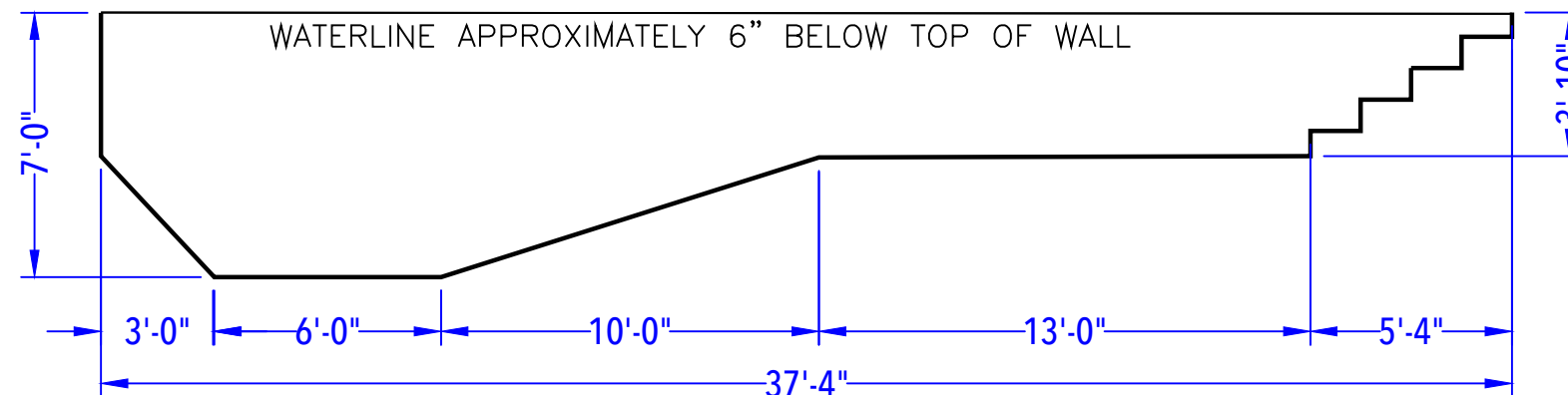
DEPTH DETAIL
