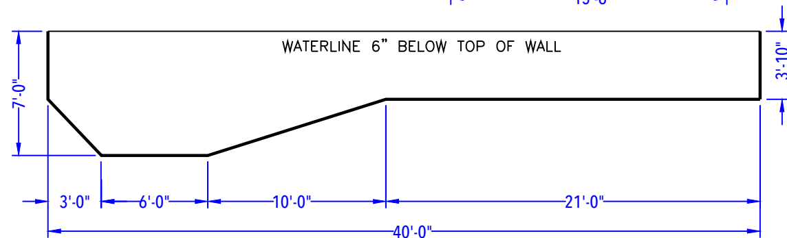
DEPTH DETAIL
