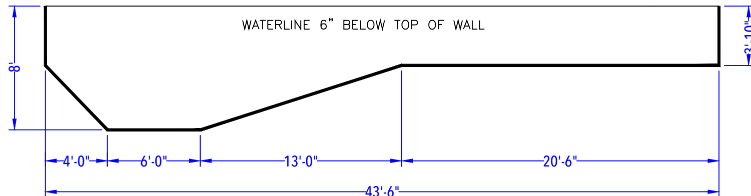
DEPTH DETAIL
