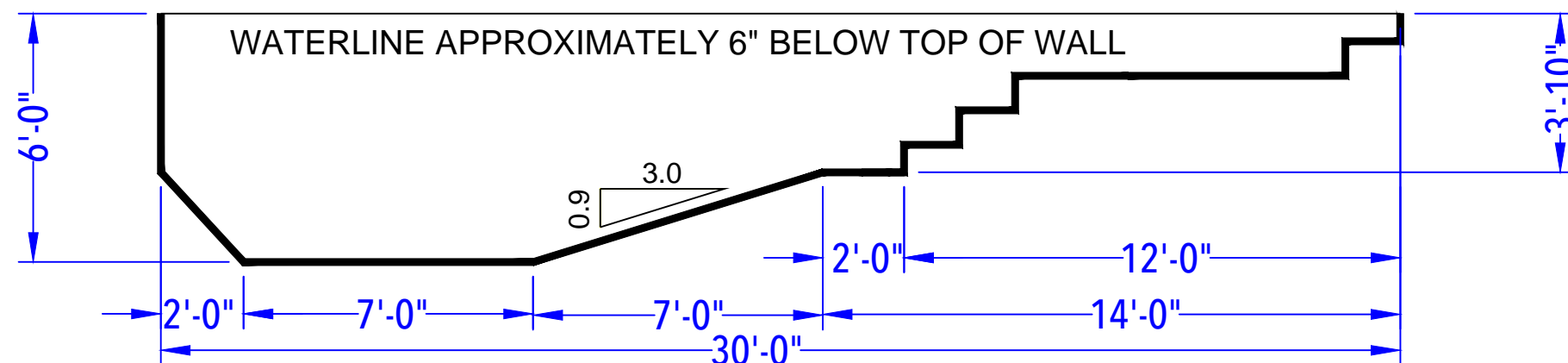
DEPTH DETAIL
