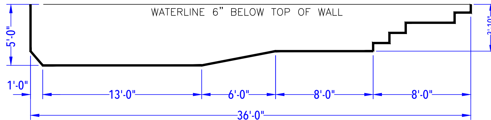
DEPTH DETAIL
