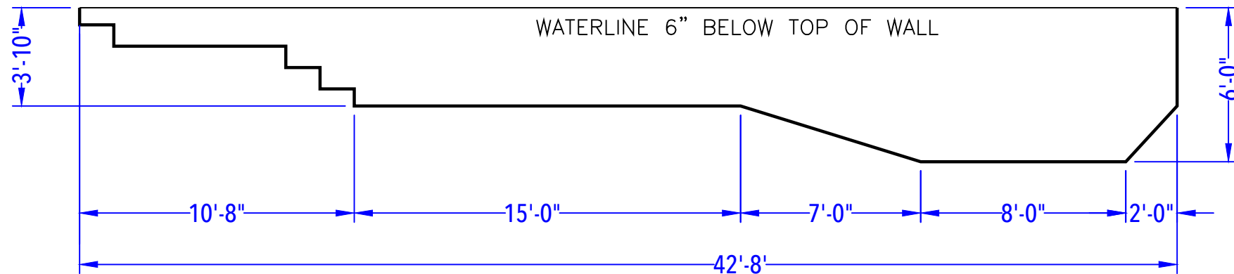
DEPTH DETAIL
