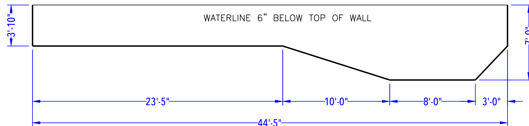
DEPTH DETAIL
