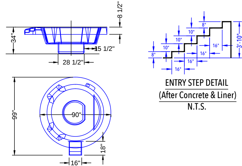
90" ROUND FIBERGLASS SPILLOVER SPA DETAIL (After Concrete & Liner) N.T.S.
