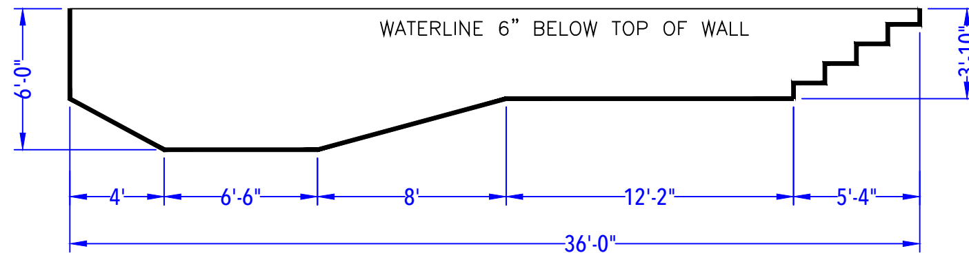
DEPTH DETAIL
