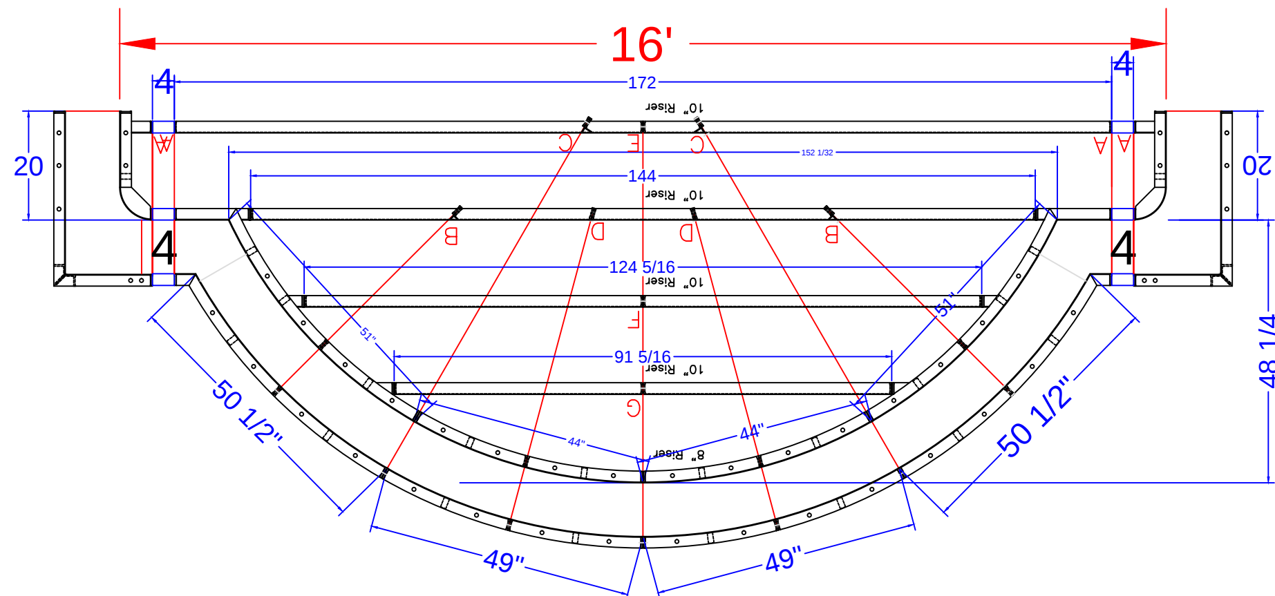
7' RADIUS ROMAN END STEP DETAIL SCALE: 1' = 1/2"
