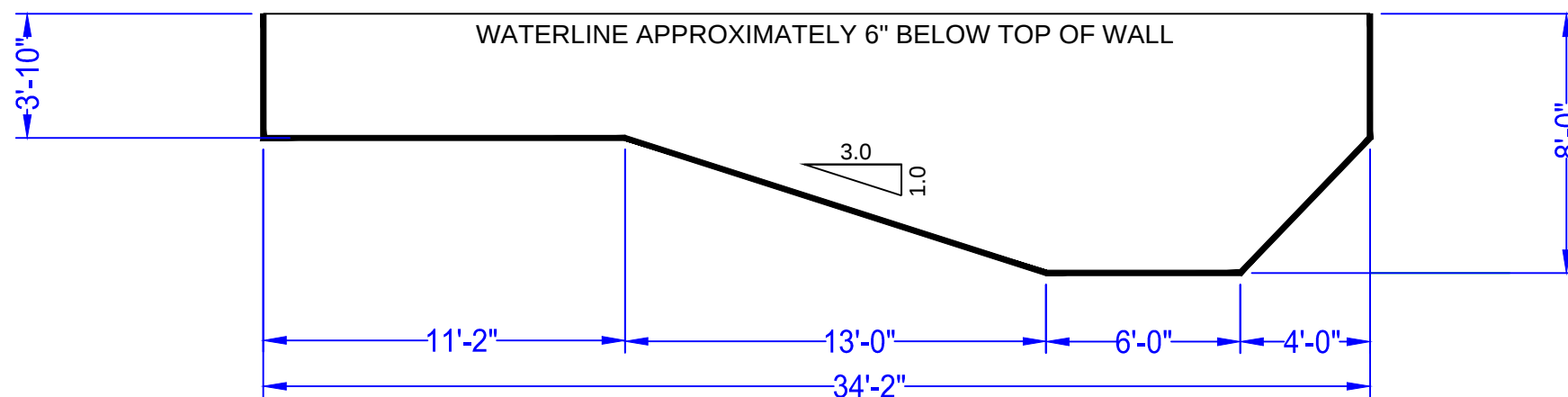
DEPTH DETAIL
