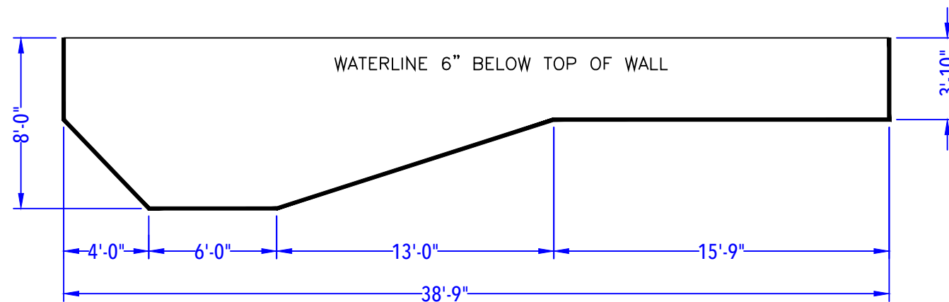
DEPTH DETAIL
