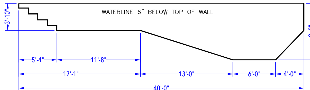
DEPTH DETAIL
